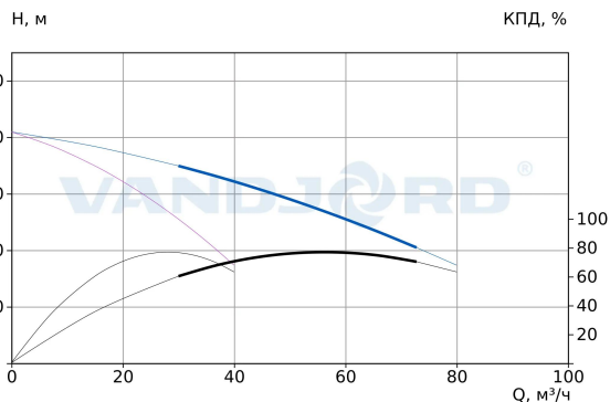
75211452 Hydro-FS-A 2/1 CRV 32-2 G2-B-100-16
