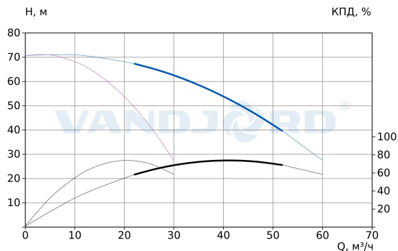
75211444 Hydro-FS-A 2/1 CRV 20-5 G2-B-100-16
