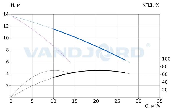
75211422 Hydro-FS-A 2/1 CRV 10-1 G2-B-80-16
