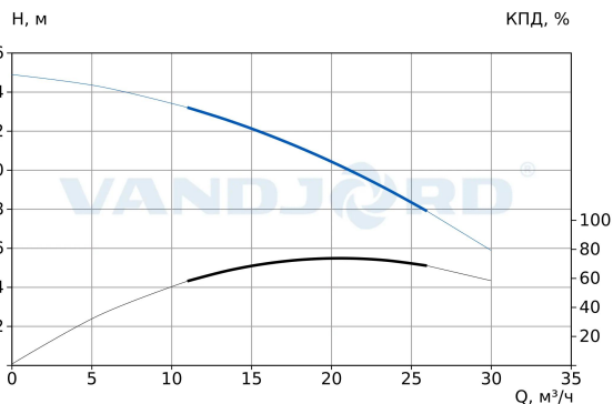
75211373 Hydro-FS-A 1/1 CRV 20-1 G2-B-80-16
