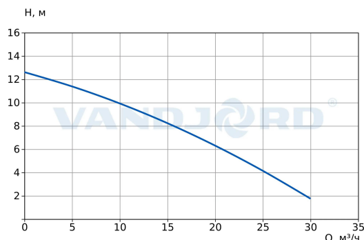
71121013 MEGA S 50-12F 1x230V
