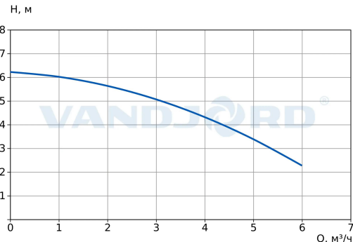
71121005 MEGA 40-6F 1x230V
