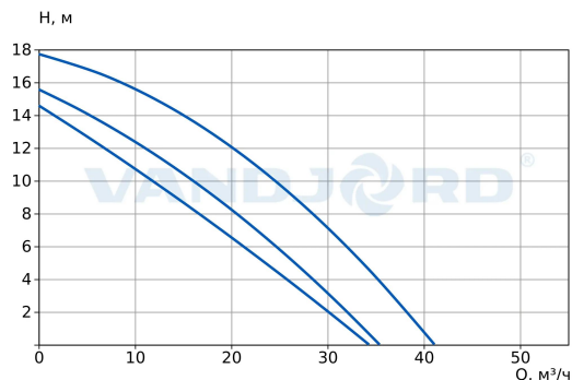
71242002 BASIC PRO 50-20SF 3x380V
