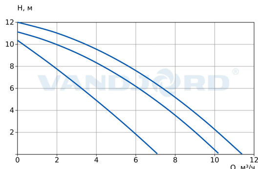
71241004 BASIC PRO 32-12SF 1x230V
