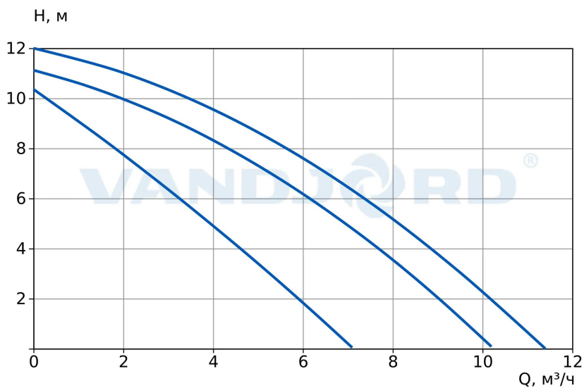
71241004 BASIC PRO 32-12SF 1x230V
