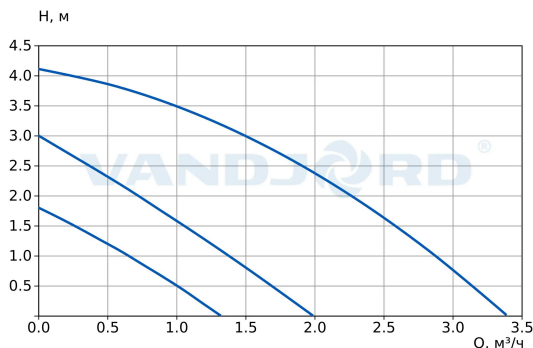
71212001 BASIC 15-4S N 130 1x230V
