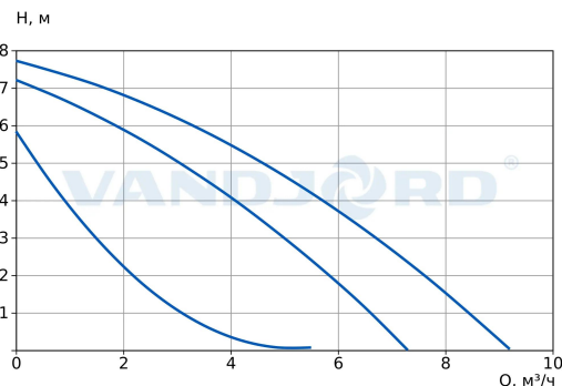
71211003 BASIC S 25-8S 180 1x230V
