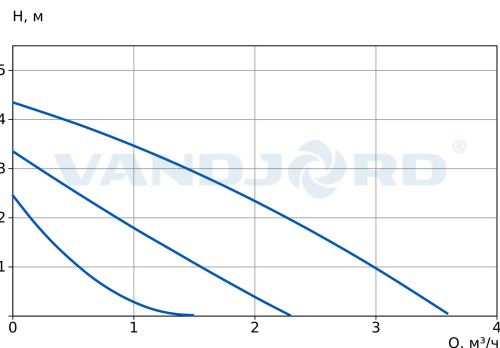
71211001 BASIC S 25-4S 180 1x230V
