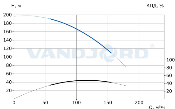
76231016 VDW.150.1100.5.1D
