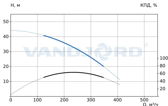
76241011 VDS.150.450.4.5.1D
