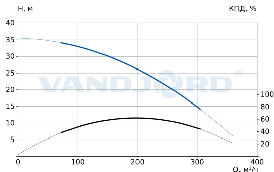
76241009 VDS.150.300.4.5.0D
