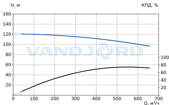
73319038 VNK 200-150/293 Q-A-E-B-AB-E
