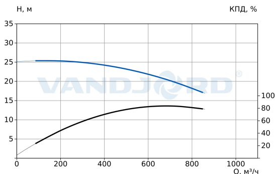
73323001 VNK 350-300/392 Q-A-E-B-AB-E
