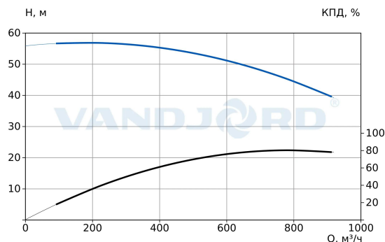
73322007 VNK 300-250/400 Q-A-E-B-AB-E
