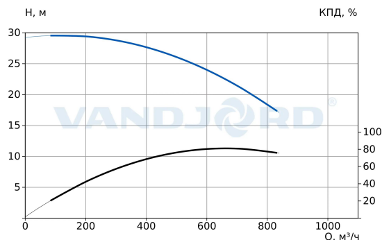
73322002 VNK 300-250/304 Q-A-E-B-AB-E
