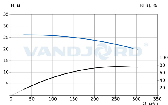
73319031 VNK 200-150/402 Q-A-E-B-AB-E
