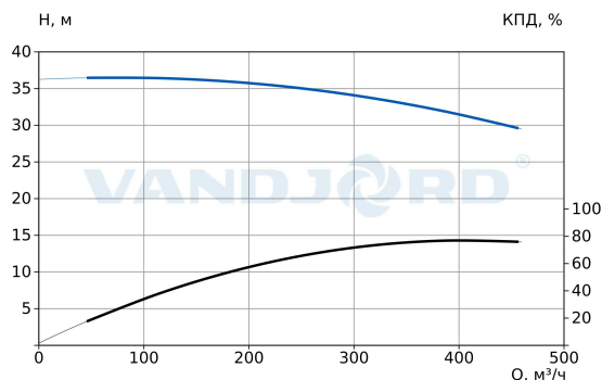
73321010 VNK 250-200/326 Q-A-E-B-AB-E
