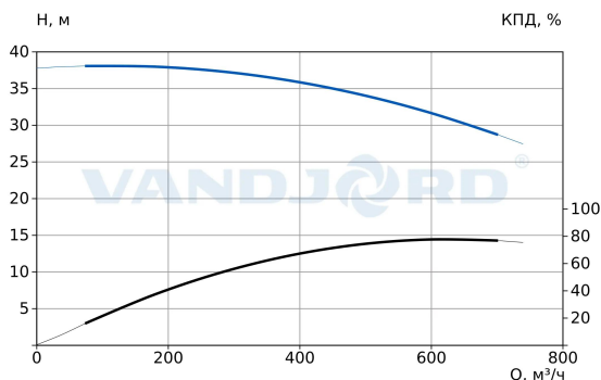
73321008 VNK 250-200/347 Q-A-E-B-AB-E
