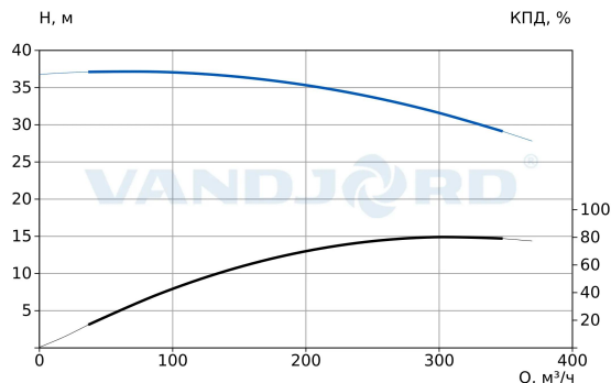
73319016 VNK 200-150/317 Q-A-E-B-AB-E
