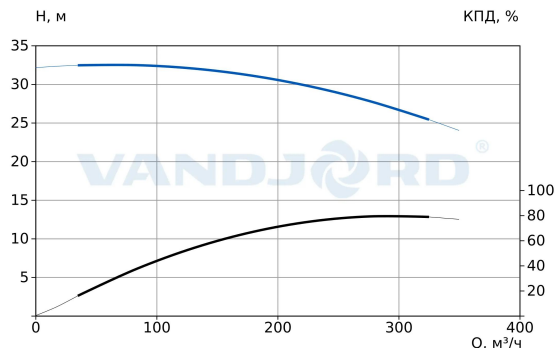
73319015 VNK 200-150/300 Q-A-E-B-AB-E
