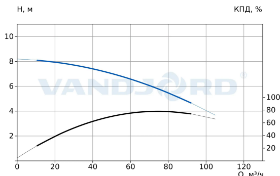
73317020 VNK 125-100/168 Q-A-E-B-AB-E
