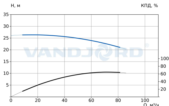
73316027 VNK 100-80/279 Q-A-E-B-AB-E
