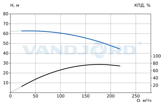
73317010 VNK 125-100/212 Q-A-E-B-AB-E
