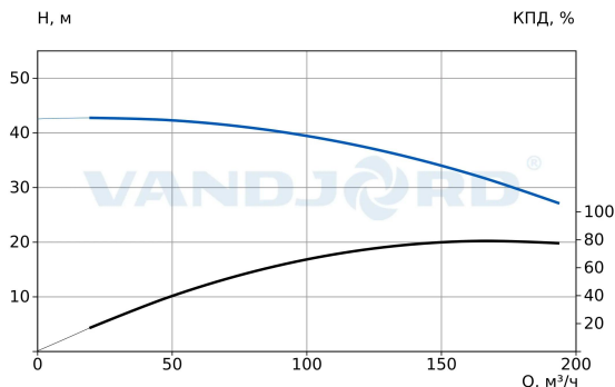
73317007 VNK 125-100/179 Q-A-E-B-AB-E
