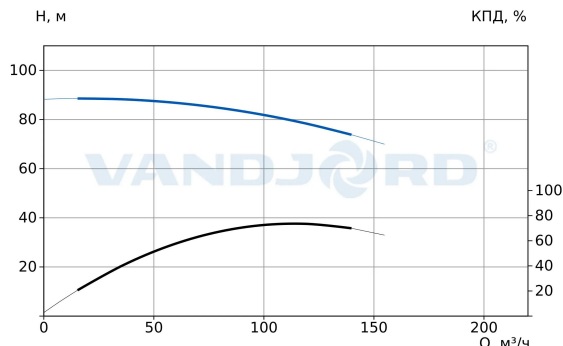
73316012 VNK 100-80/242 Q-A-E-B-AB-E
