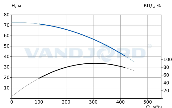
73217077 NBV iNOX 125-200-90/2 CN-A1-D-E-B-A-E
