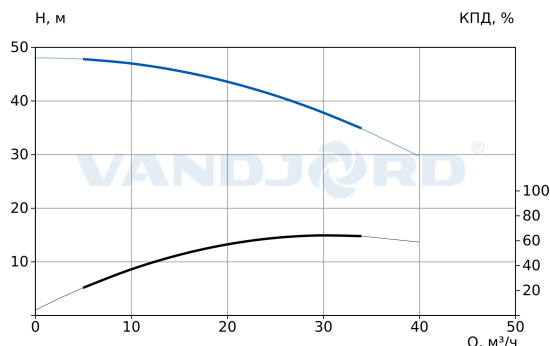
73212046 NBV iNOX 40-200-5.5/2 CN-A1-D-E-B-A-E
