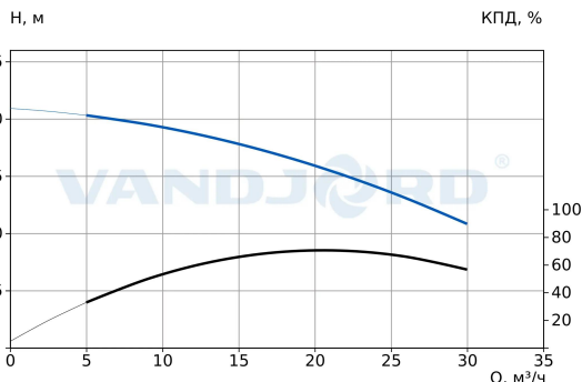
73212042 NBV iNOX 40-125-1.5/2 CN-A1-D-E-B-A-E
