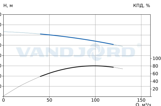
73214069 NBV iNOX 65-200-22/2 CI-A1-D-E-B-A-E
