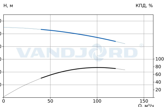
73214068 NBV iNOX 65-200-18.5/2 CI-A1-D-E-B-A-E
