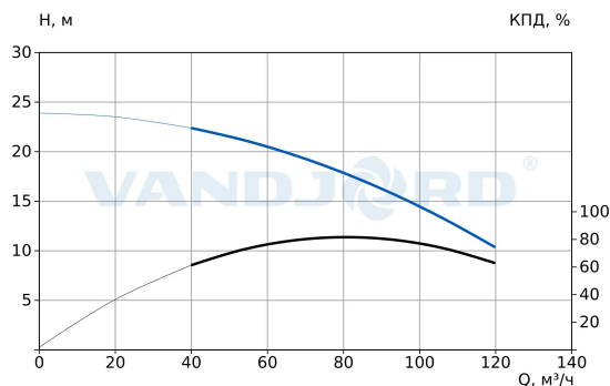
73214063 NBV iNOX 65-125-5.5/2 CI-A1-D-E-B-A-E
