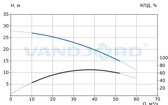
73213057 NBV iNOX 50-125-4/2 CI-A1-D-E-B-A-E
