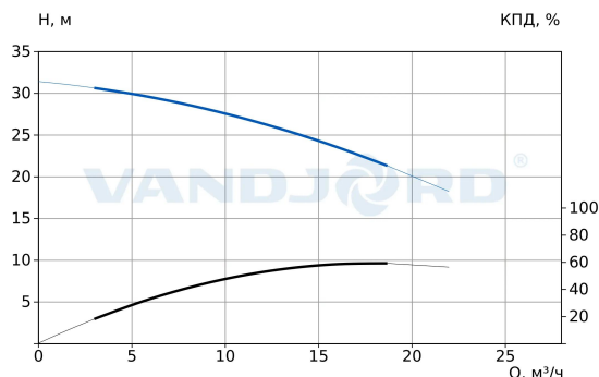
73211028 NBV iNOX 32-160-2.2/2 CI-A1-D-E-B-A-E
