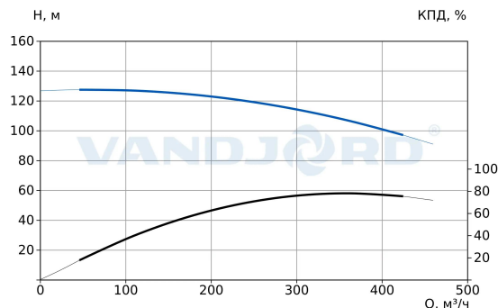
73217021 NBV 125-303-160/2 Q-B-D-E-B-A-E
