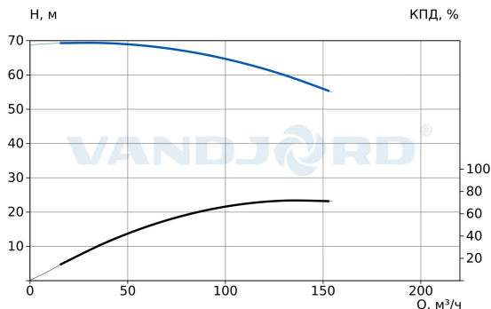
73215031 NBV 80-220-37/2 Q-A-D-E-B-A-E
