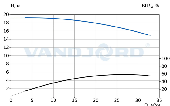
73213038 NBV 50-230-2.2/4 Q-A-D-E-B-A-E
