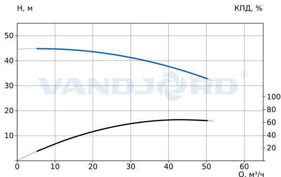
73213030 NBV 50-175-7.5/2 Q-A-D-E-B-A-E
