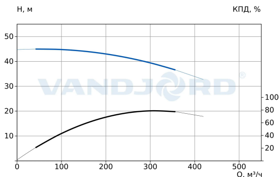
73119132 TPV 150-410-45/4 Q-A-BT-E
