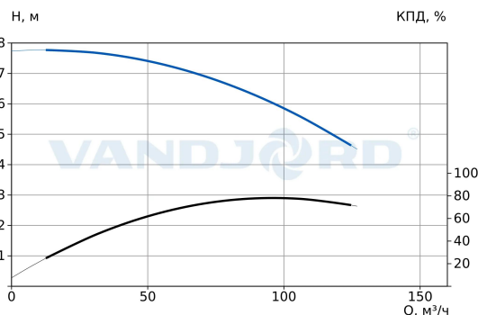
73118142 TPV 125-60-2.2/4 Q-A-BT-E
