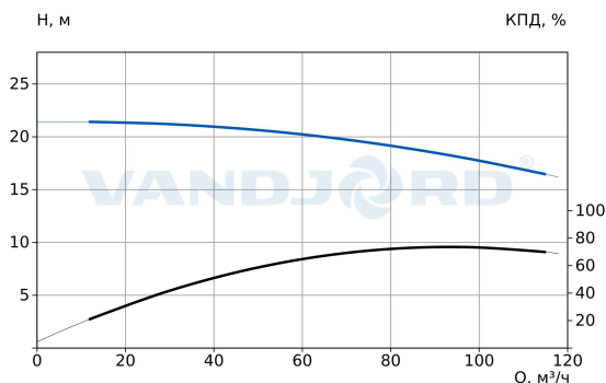
73117158 TPV 100-180-7.5/4 Q-A-BT-E
