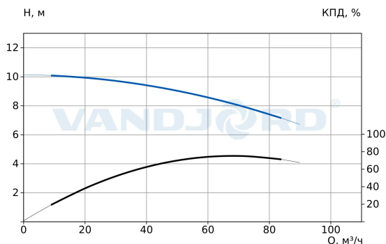
73117154 TPV 100-80-2.2/4 Q-A-BT-E
