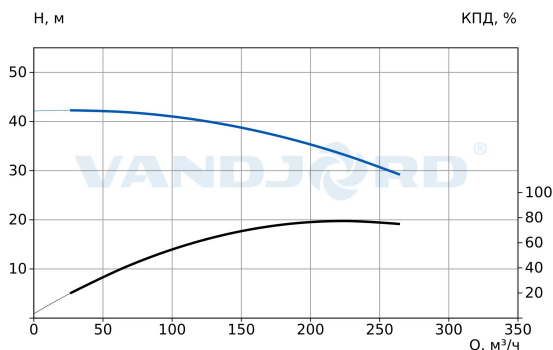
73118131 TPV 125-330-30/2 Q-A-BT-E
