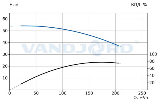
73117140 TPV 100-450-30/2 Q-A-BT-E
