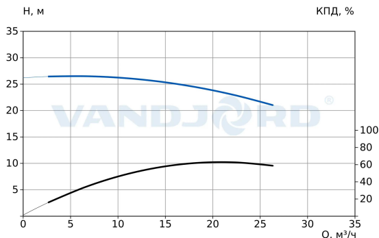
73113114 TPV 40-230-2.2/2 Q-A-BT-E
