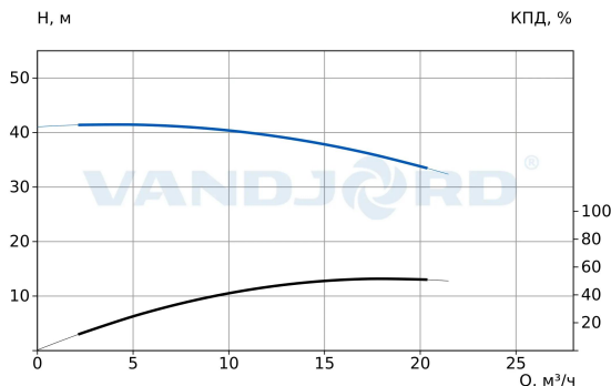
73112115 TPV 32-360-4/2 Q-A-BT-E
