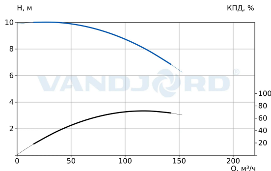
73118127 TPV 125-80-4/6 Q-A-B-E
