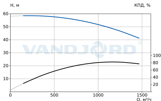
73124121 TPV 350-470-220/4 Q-A-B-E
